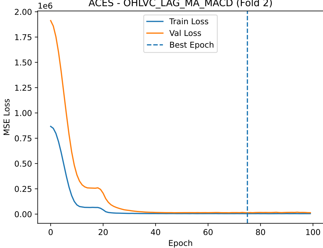
ACES - OHLVC_LAG_MA_MACD (Fold 2)
